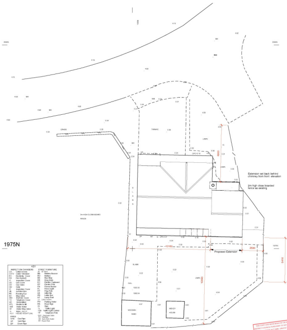
Roof Plan and Site 1:100
