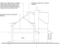
East Elevation
