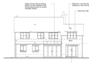
South Elevation
